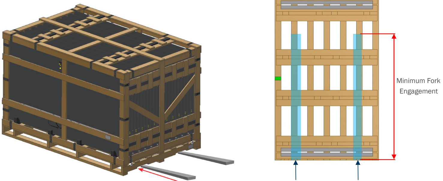
Figure 4: Series 7 TR1 Short Side Forklift Engagement
