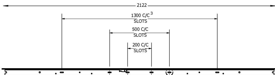
Figure 8: Slot Distance from Backrail Centerline. The nominal rail thickness is 0.89 3 /1.09mm
