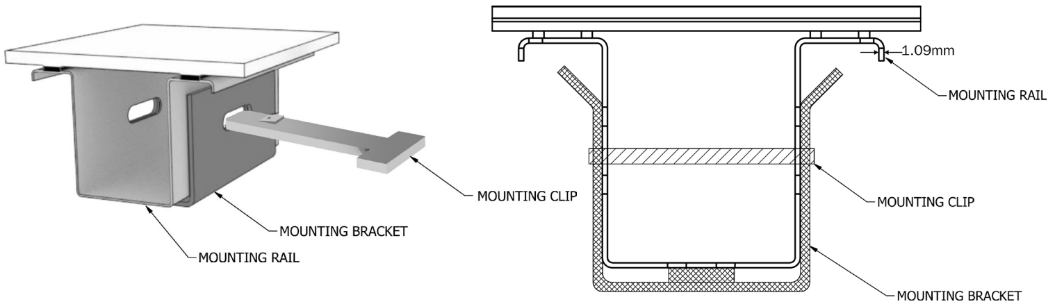
Figure 6: Bracket and Clip Mounting Details
