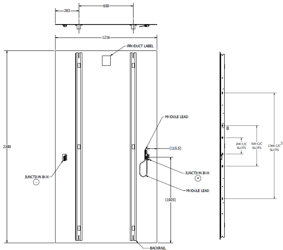
Figure 5: Series 7 Module Mechanical Drawing
