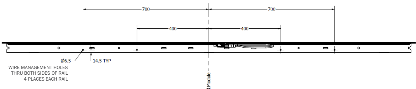
Figure 10: Wire Management Hole Dimensions
