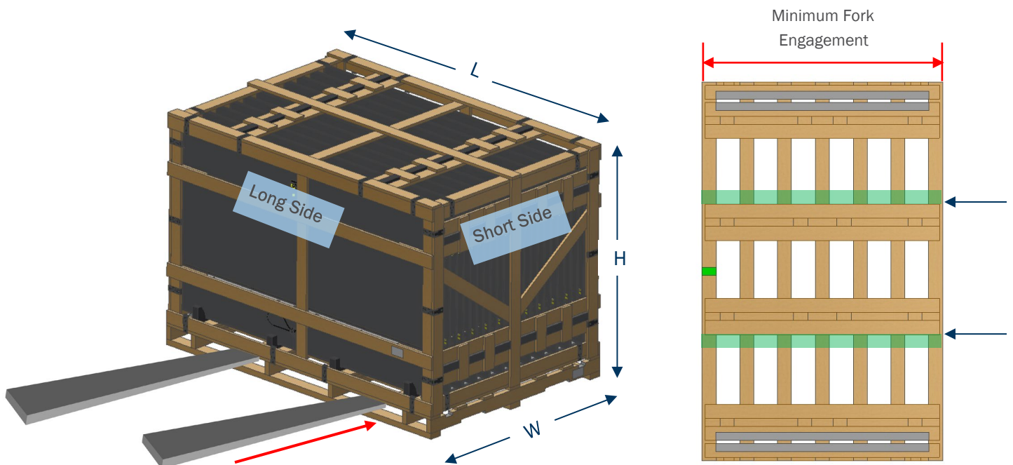
Figure 3: Series 7 TR1 Long Side Forklift Engagement
