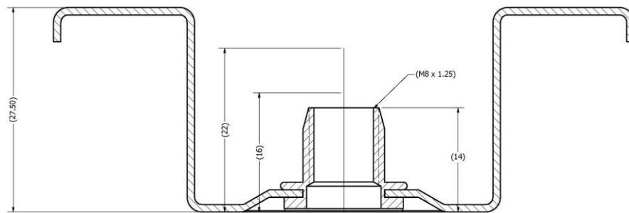
Figure 5: Cross sectional view of module back rail
