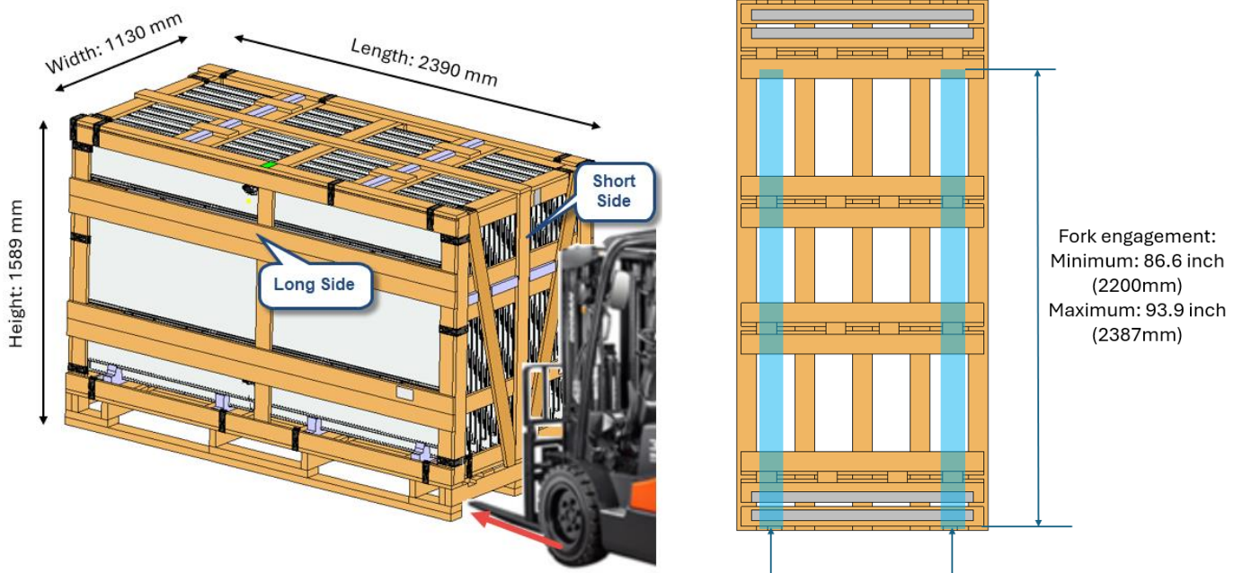
Figure 2: Series 7 FT1 short side forklift engagement
