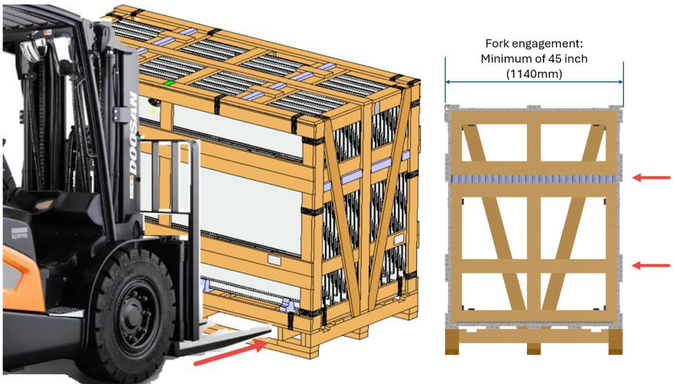
Figure 3: Series 7 FT1 long side forklift engagement
