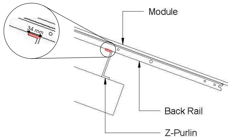
Figure 8: Mounting structure Z-purlin minimum width
