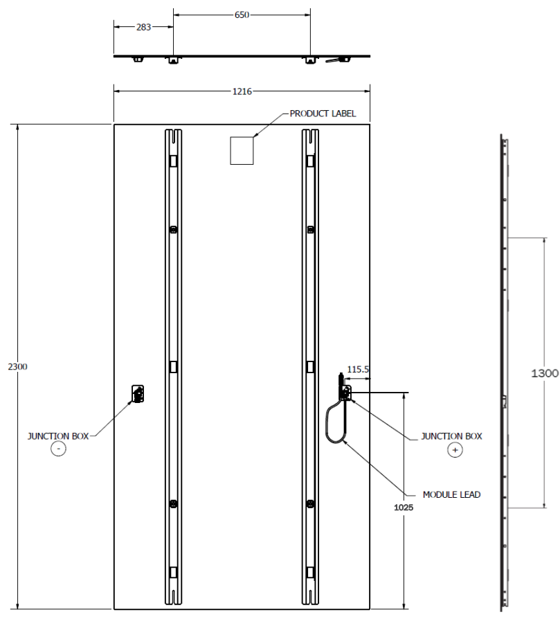
Figure 4: Series 7 FT1 module mechanical drawing. All dimensions are in mm.
