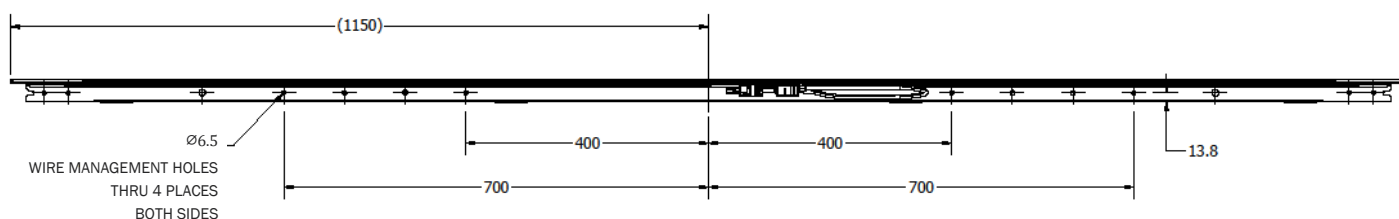
Figure 11: Wire management hole dimensions
