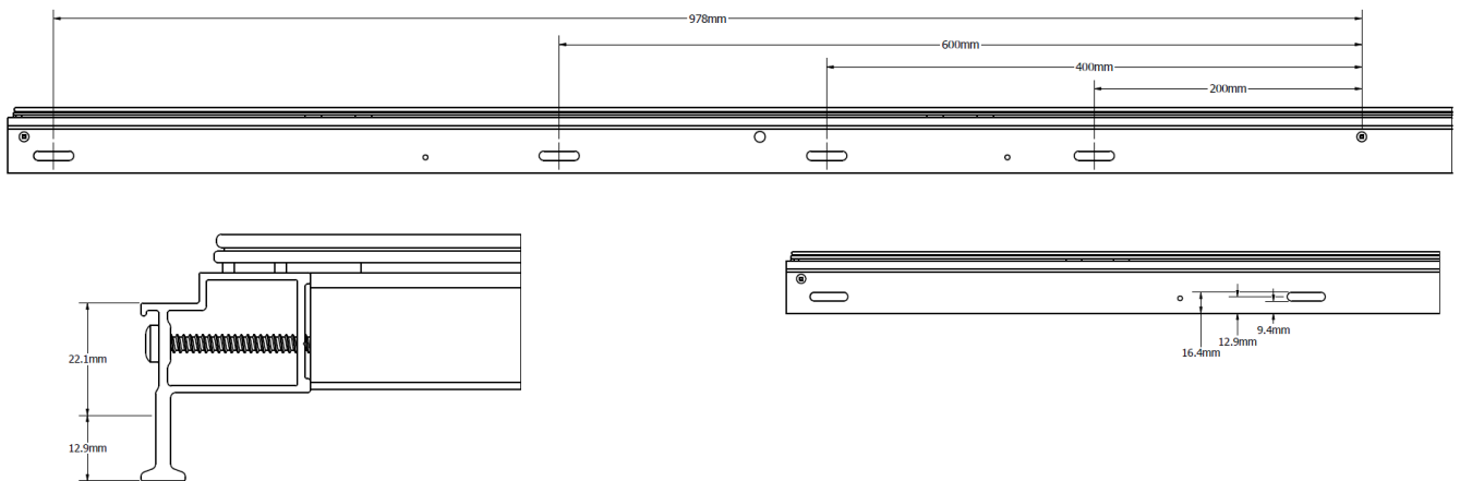
Figure 8: SpeedSlot/Corner Slot Hole Detail on Long Edge Frame
