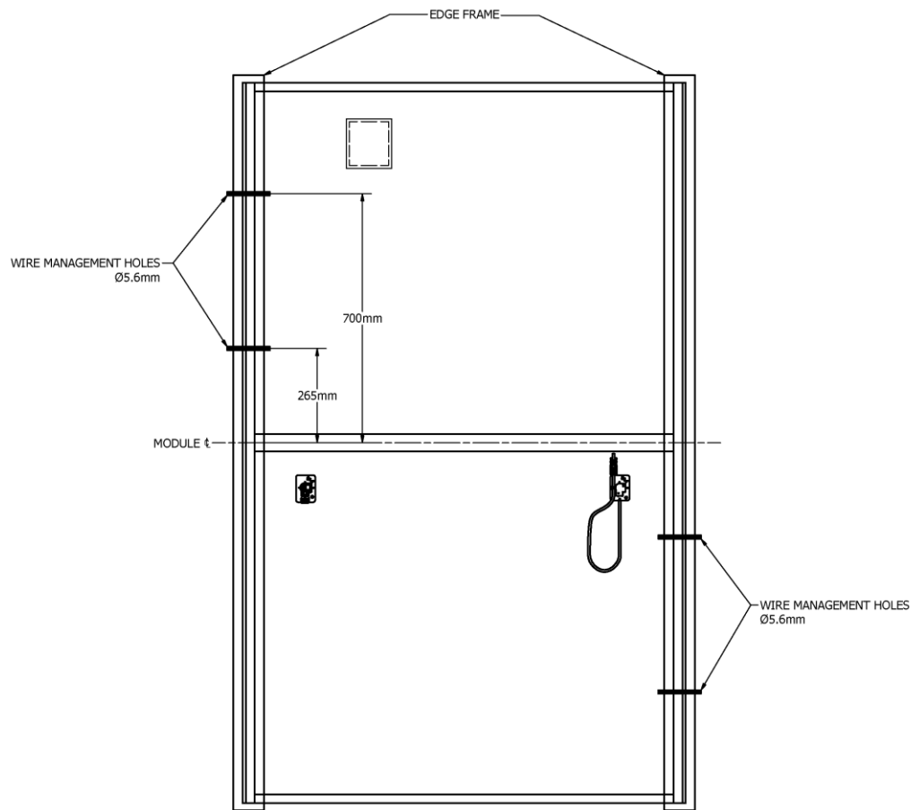
Figure 12: Frame Wire Management Hole Locations
