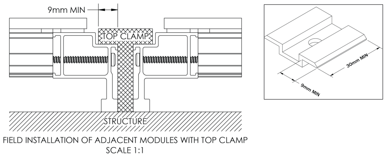
Figure 6: Shared Top Clamp Detail
