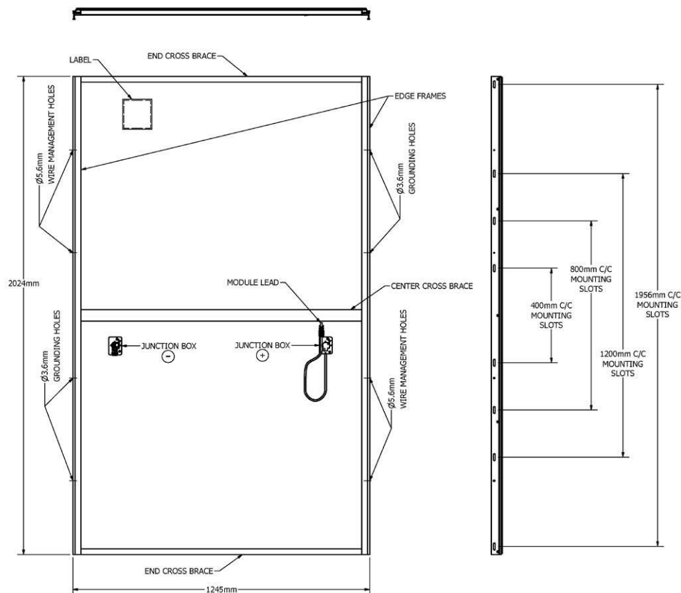
Figure 5: Series 6 Plus V2 Module Mechanical Drawing Showing the Backside
