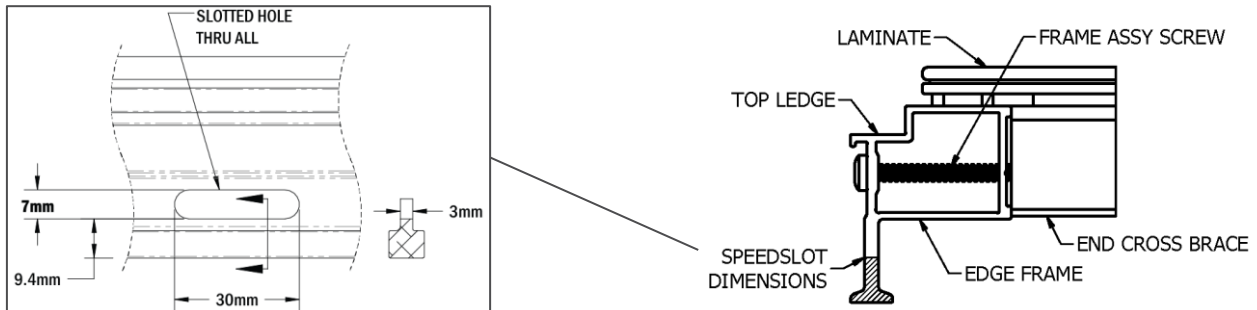
Figure 7: SpeedSlot Hole Dimensions
