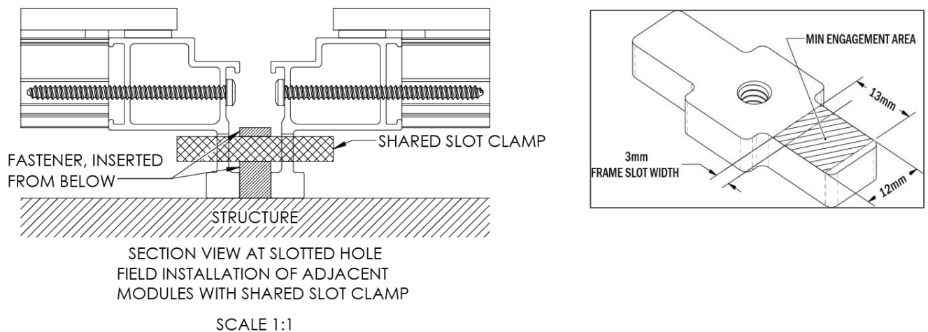
Figure 9: Shared SpeedSlot Clamp Detail
