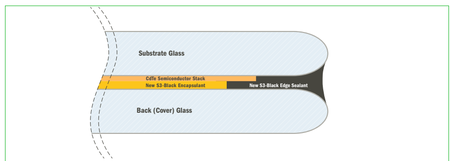
Figure 1. Cross section of First Solar’s S3 Black and S3 Black Plus modules.
