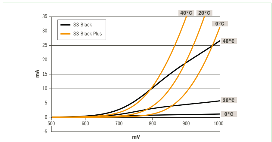
Figure 9. Comparison of the I - V curves of S3 Black (standard) and S3 Black Plus (ZnTe).
