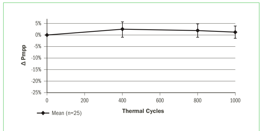
Figure 6. Results of extended thermal cycling.
