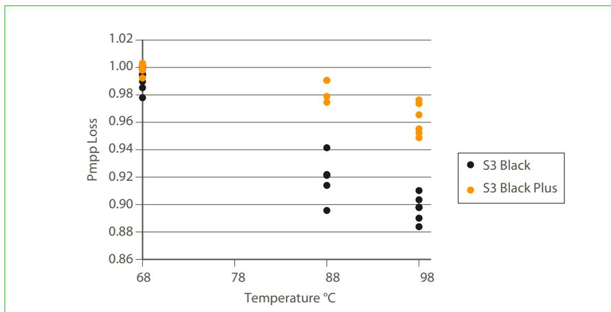
Figure 12. Comparative power loss vs. accelerated temperature stresses.
