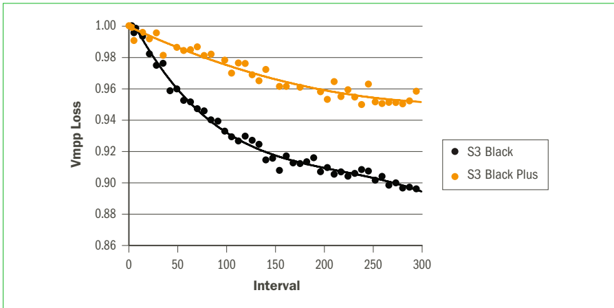
Figure 13. Voltage loss after accelerated MPP (maximum power point) light soak exposure.
