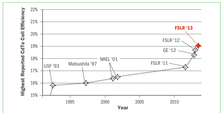
Figure 7. World-record CdTe cell efficiency (reproduced from Gloeckler et al. [18]).
