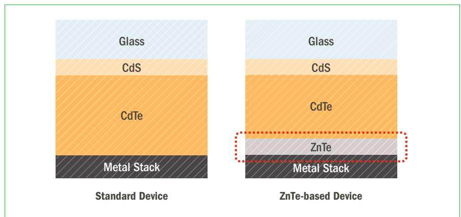
Figure 8. S3 Black (standard) and S3 Black Plus (ZnTe-based) device stack comparison.
