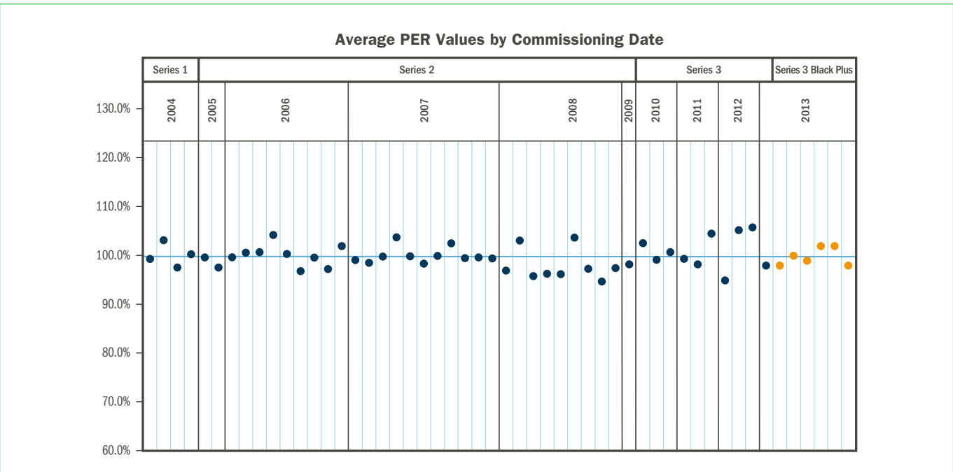
Figure 14. Performance predictability of ZnTe back-contact modules.
