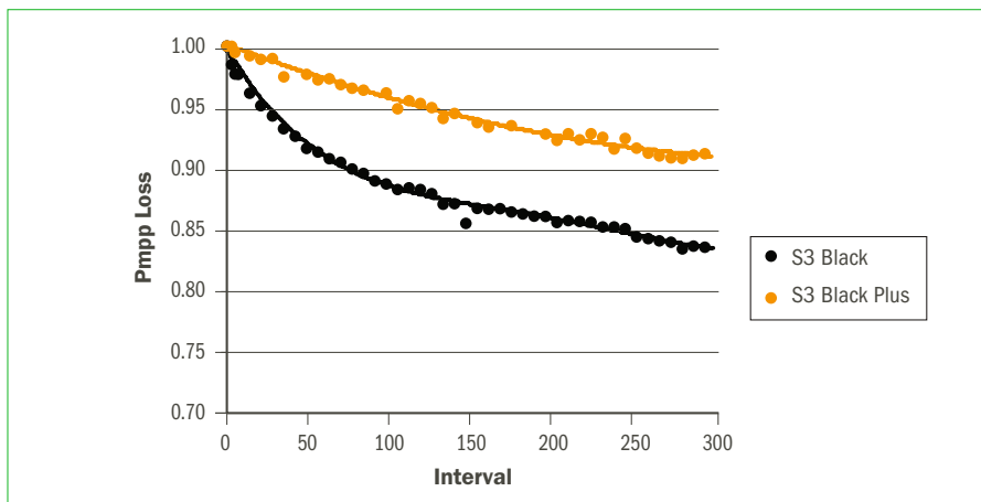
Figure 11. Power loss after accelerated light soak exposure.
