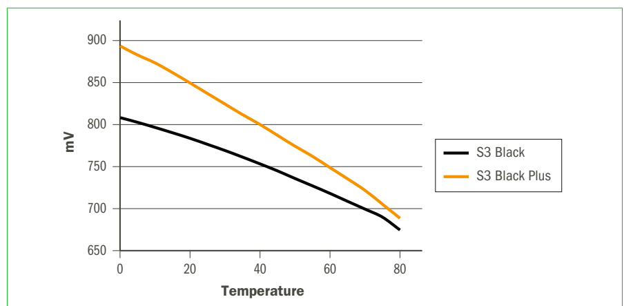
Figure 10. Comparison of back-contact V_{oc} behaviour vs. temperature.
