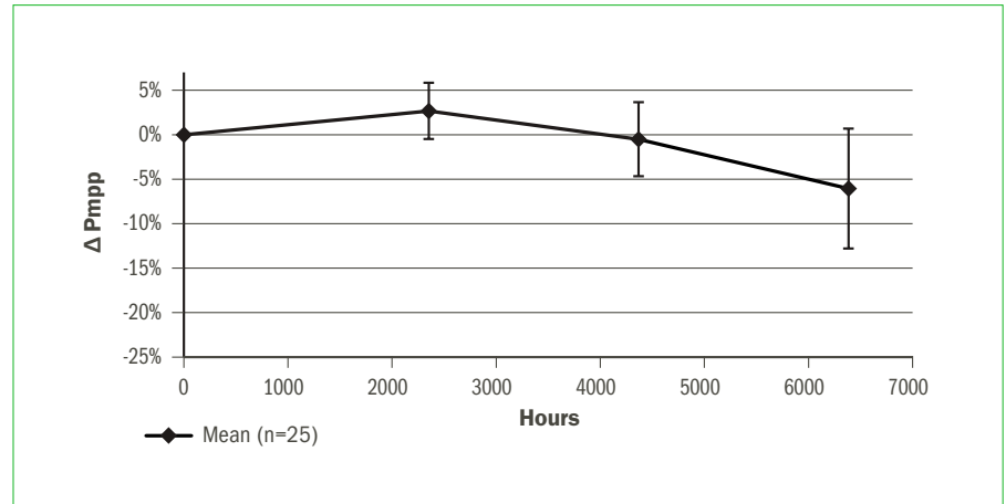
Figure 5. Results of extended damp-heat testing.
