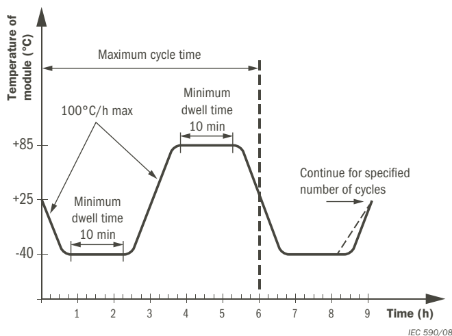
Figure 2. IEC 61646 thermal-cycling profile.
