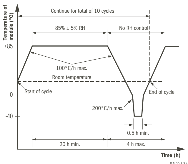
Figure 3. IEC 61646 humidity-freeze profile.
