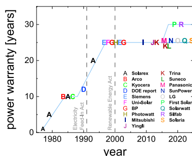
Figure 1. Warranties for PV modules over time
