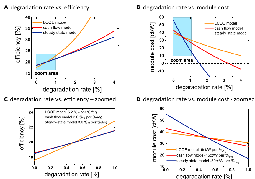
Figure 3. Comparison of constant values for the figures of merit in each model
