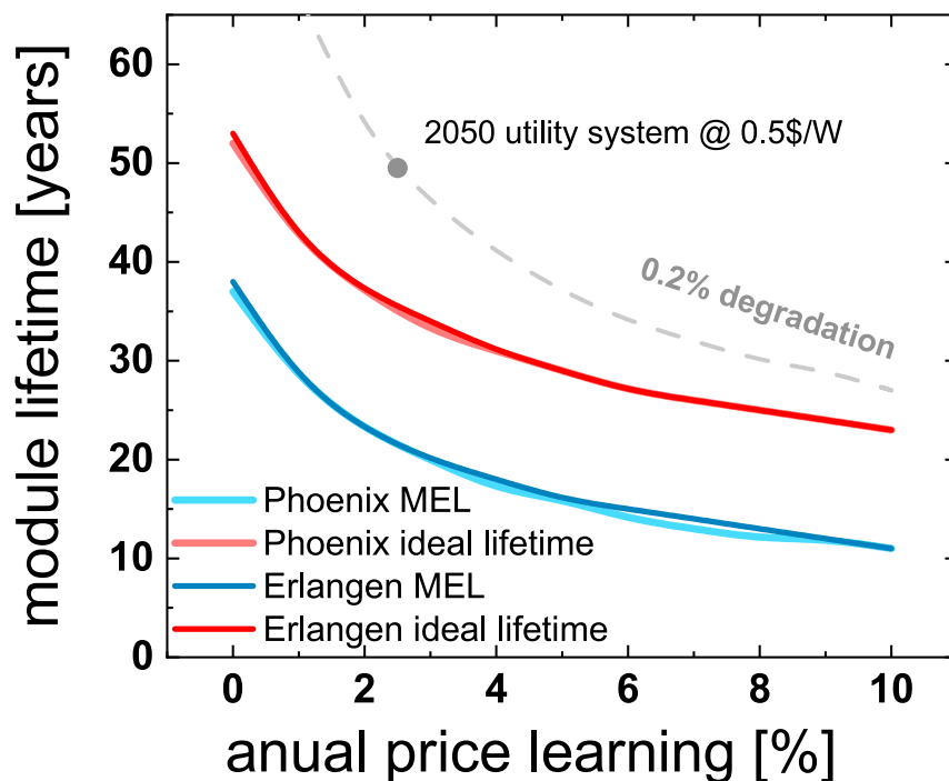
Figure 8. Cost reduction and lifetime
