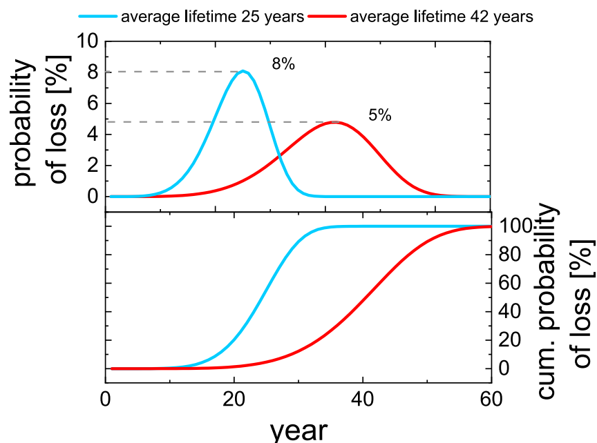
Figure 10. Probability of PV module loss
