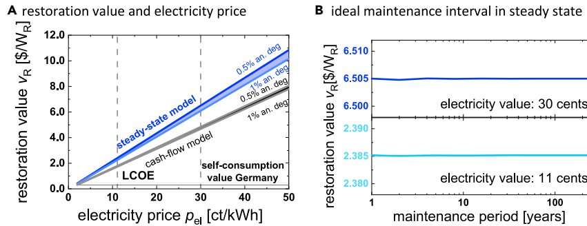
Figure 6. Value and ideal timing of maintenance in the steady-state model
