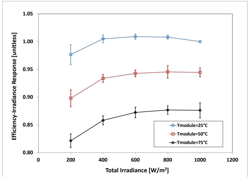
Figure1. Dependence of maximum power P_{MAX} on total irradiance and module temperature. All values are calculated with respect to P_{MAX} at standard test conditions. Error bars indicate +/- two standard deviations about the mean of response of the sample population.
