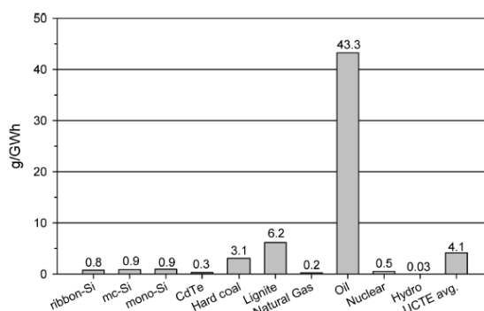
FIGURE 3. Life-cycle atmospheric Cd emissions for PV systems from electricity and fuel consumption, normalized for a Southern Europe average insolation of 1700\text{ kWh}/\text{m}^2/\text{yr} , performance ratio of 0.8, and lifetime of 30 yrs. Ground-mounted BOS (18) is assumed for all PV systems; comparisons with other electricity generation options.
