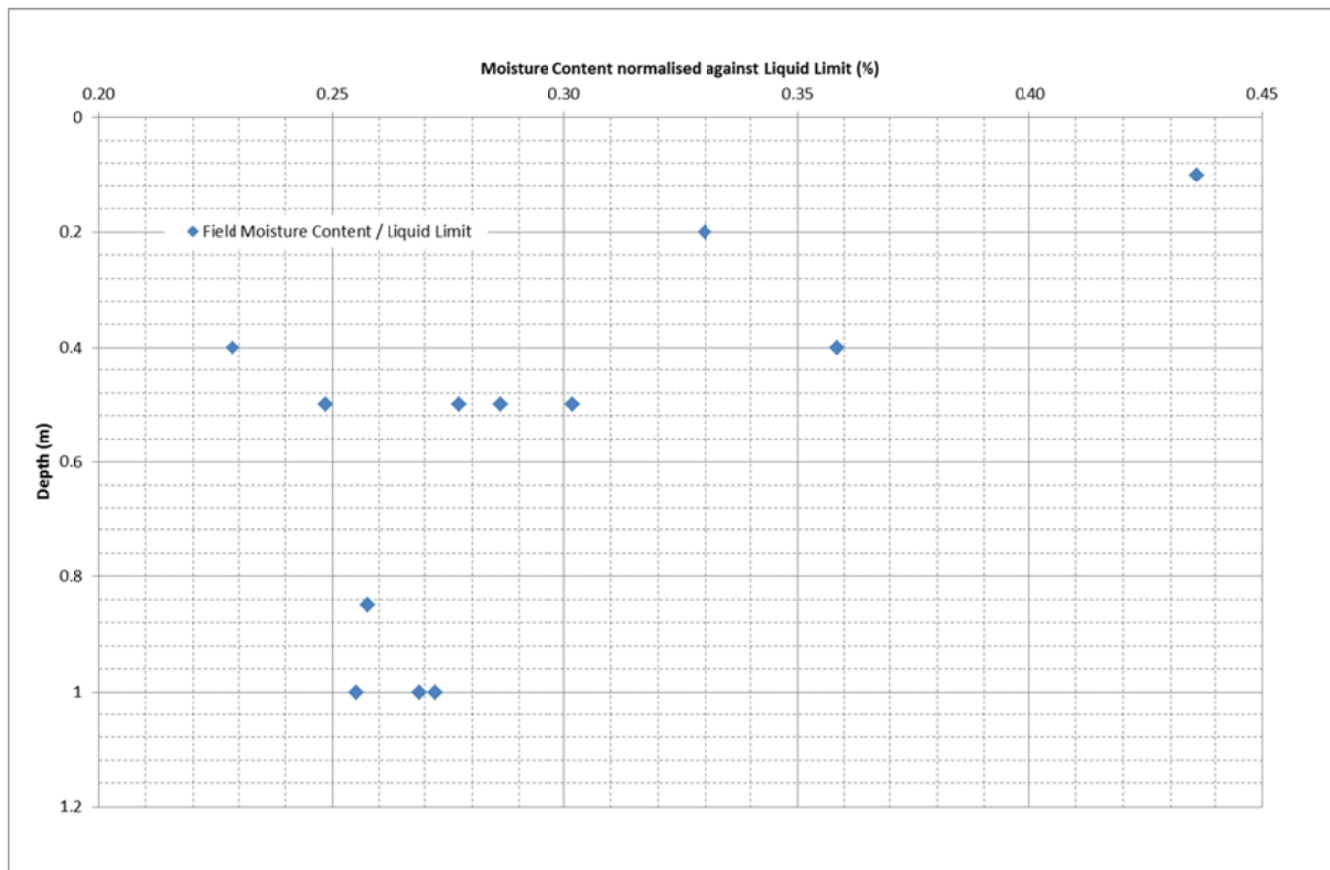
Figure 7: Field moisture content normalised against liquid limit with depth
