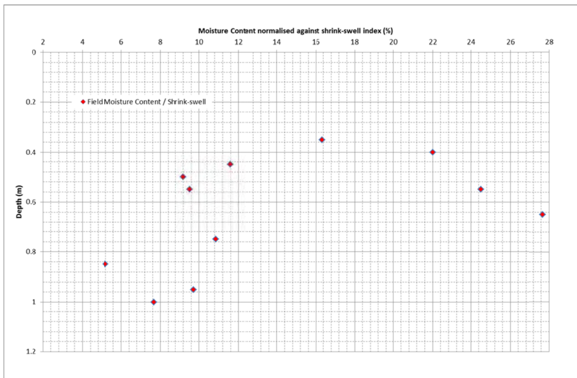
Figure 9: Field moisture content normalised with shrink-swell index against depth
