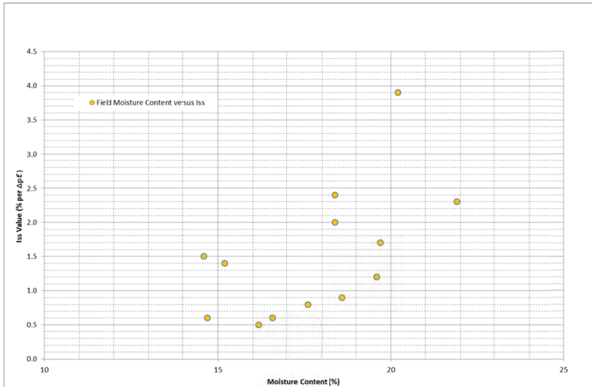
Figure 8: Moisture content versus Iss value
