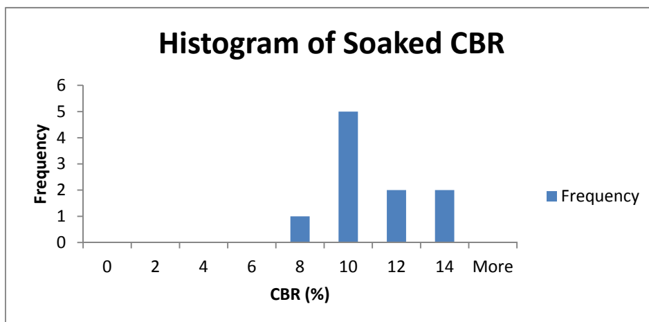
Figure 4: Histogram of Soaked CBR results
