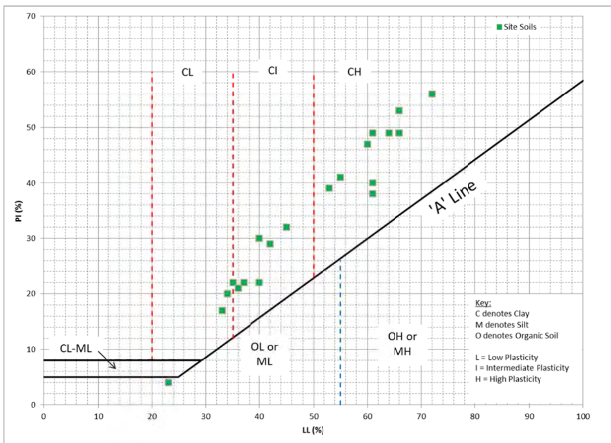
Figure 1: Results of Atterberg limit determinations
