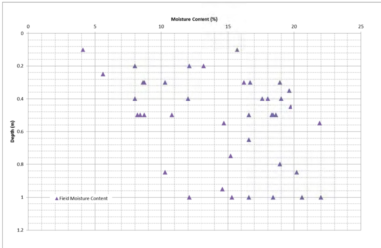
Figure 6: Field moisture content versus depth of sample
