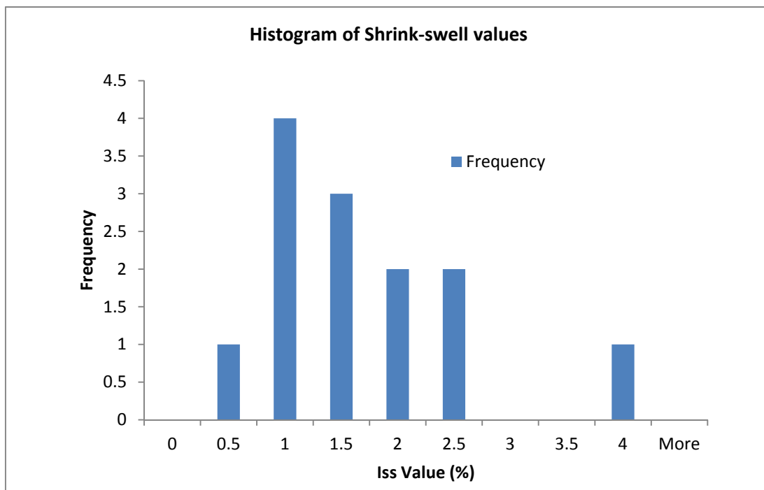
Figure 5: Histogram of Shrink-swell testing results
